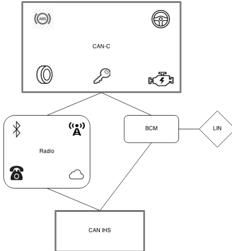
Figure 2: 2014 Jeep Cherokee architecture diagram
