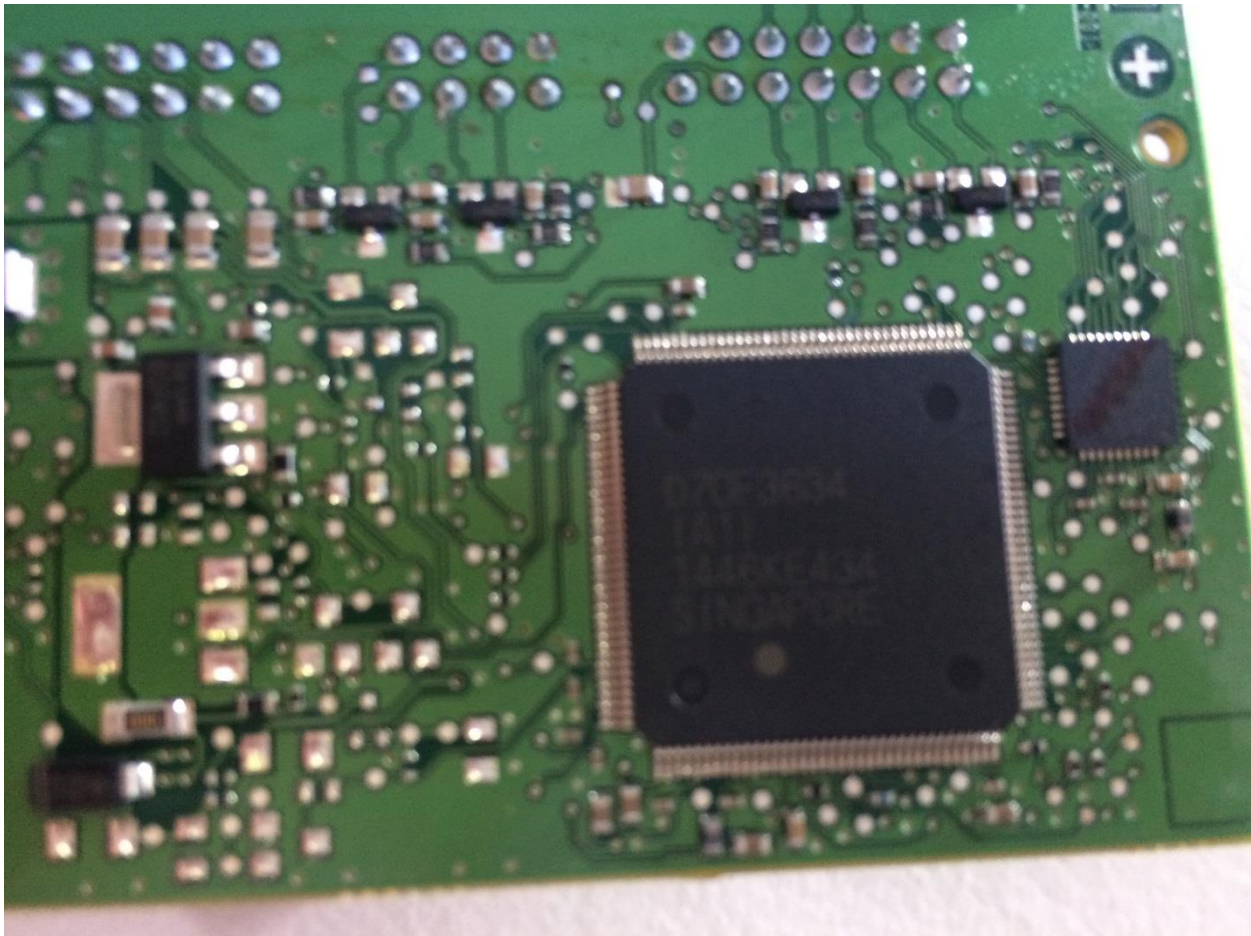
Figure 55: PAM PCB
