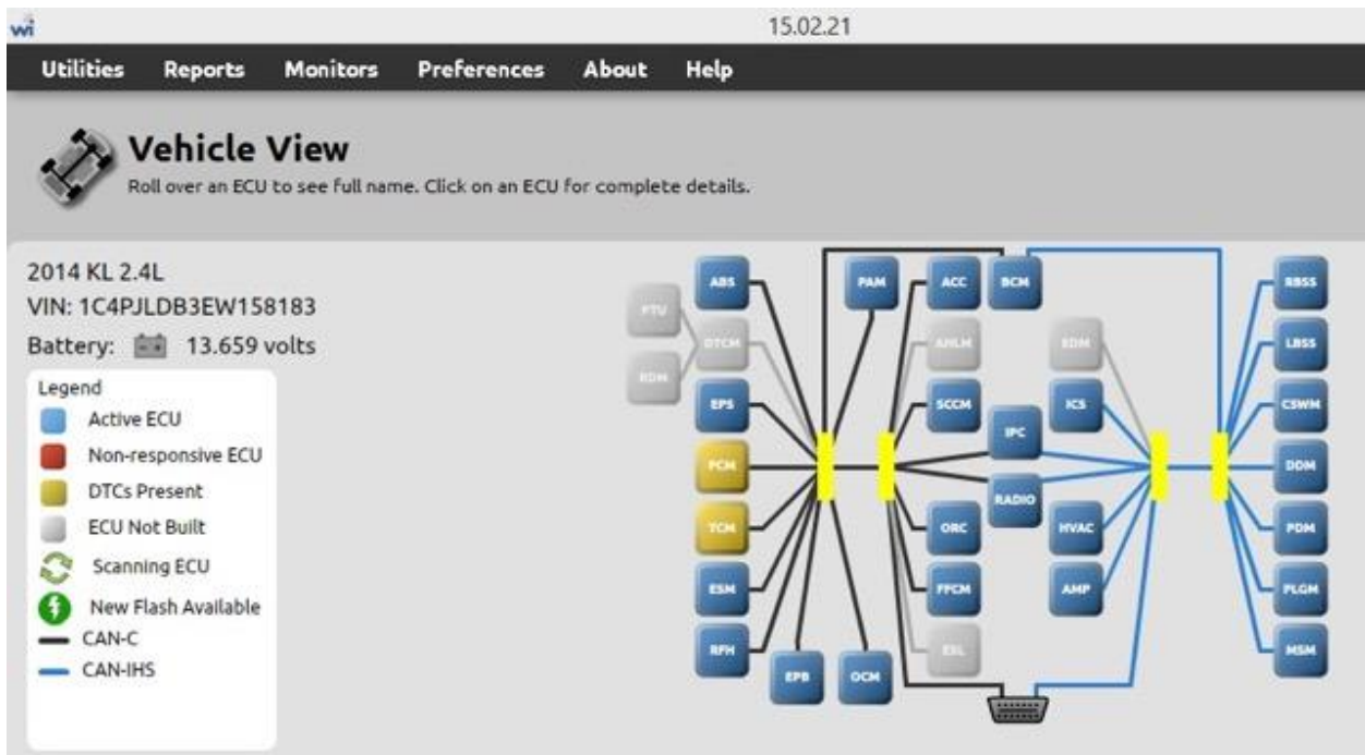
Figure 46: 2014 Jeep Cherokee ECU diagram from the WiTech software
